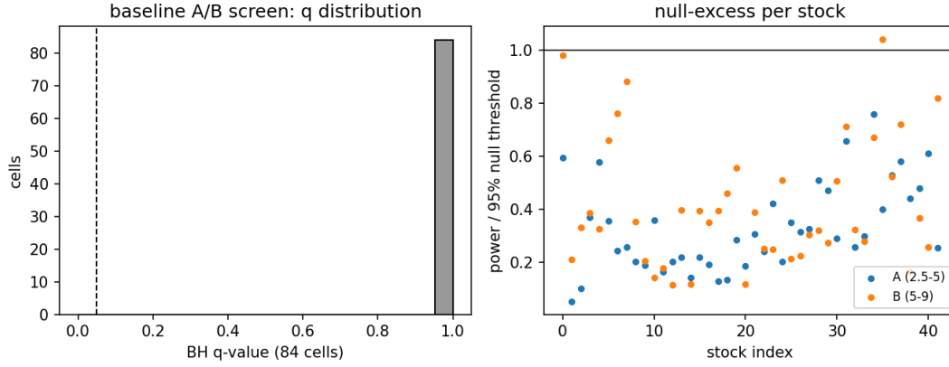
Figure 5: Baseline screen diagnostics. Left: Benjamini–Hochberg q -values over the 84 target-band cells (dashed line: 0.05; no cell significant). Right: per-stock band power relative to the 95% per-stock AR(1) threshold in bands A and B (horizontal line: unity).
